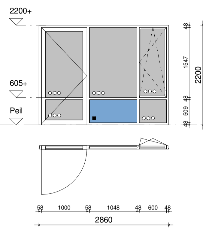
merk A0.01 - aluminium, Reynaers type SL 38 Cubic
